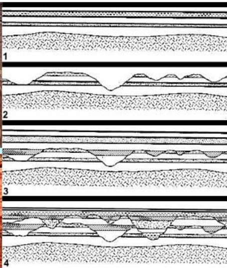
Left: Erosion in sediments from around the world.
